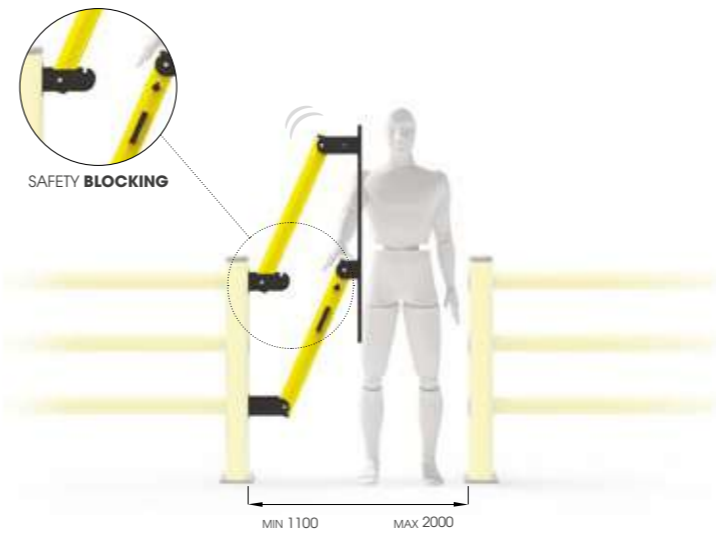
LIFT GATE 150
